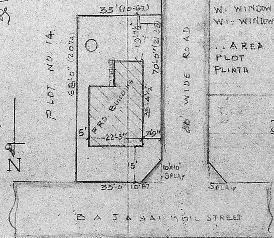
SITE PLAN SCALE 1"=24'-0"
