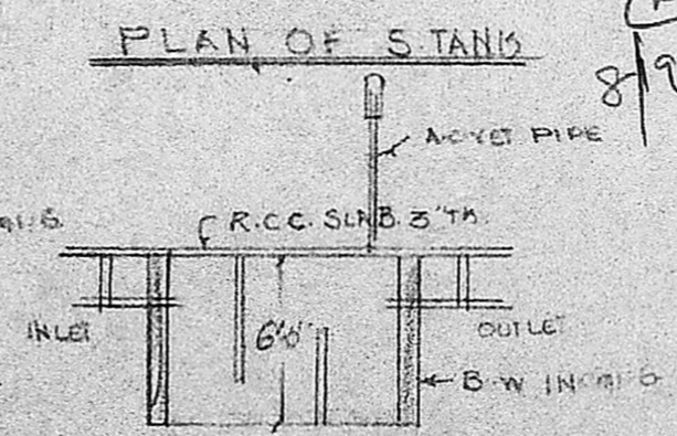
SECTION OF PLAN
